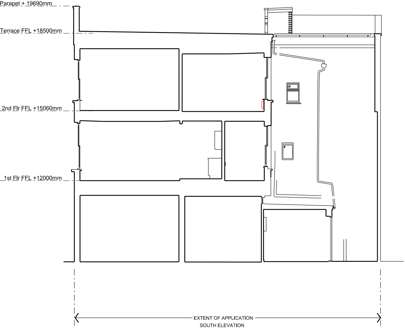
02 SOUTH ELEVATION
