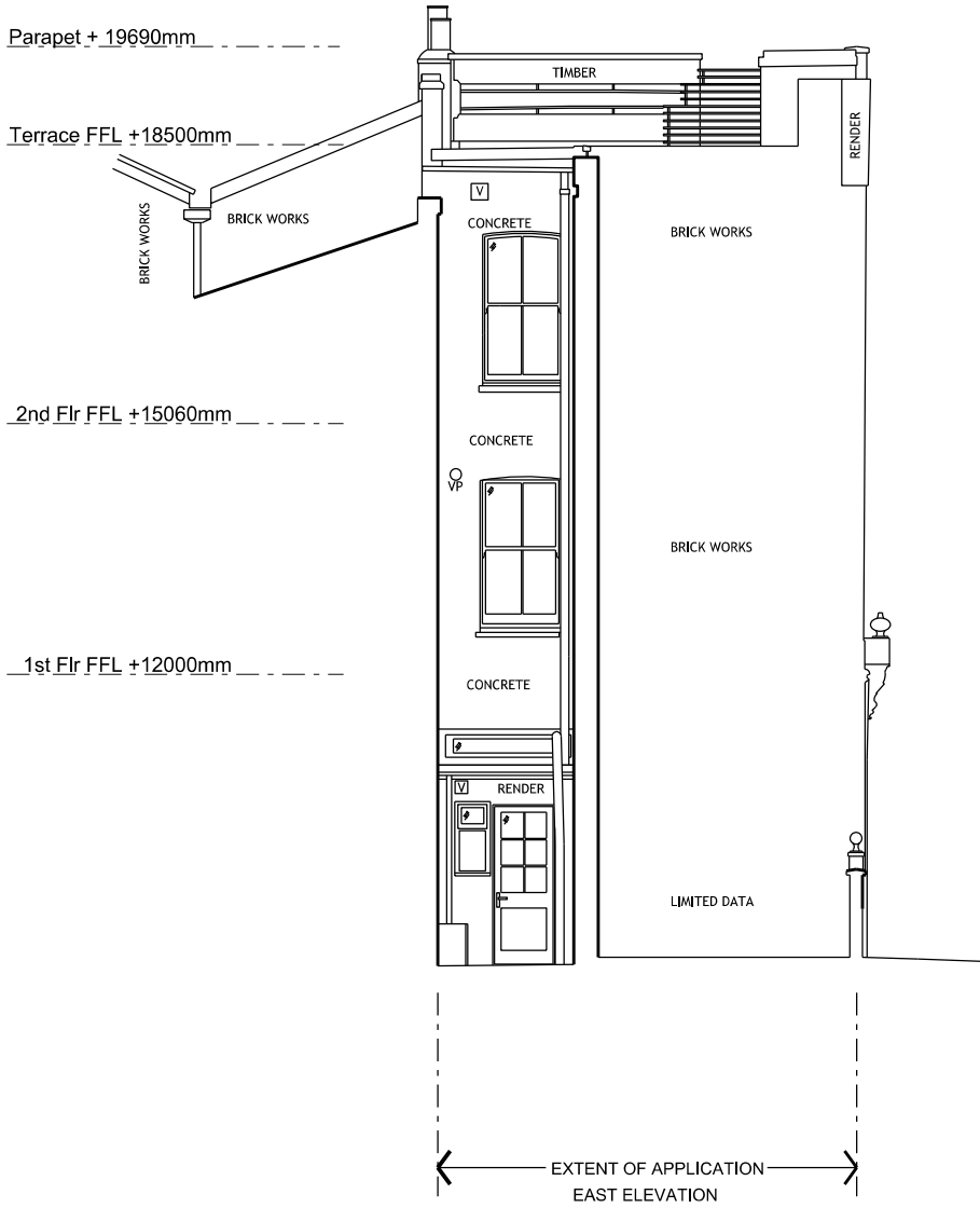
01 EAST ELEVATION
