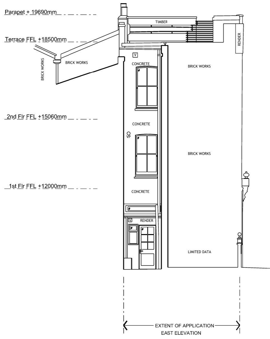
01 EAST ELEVATION
