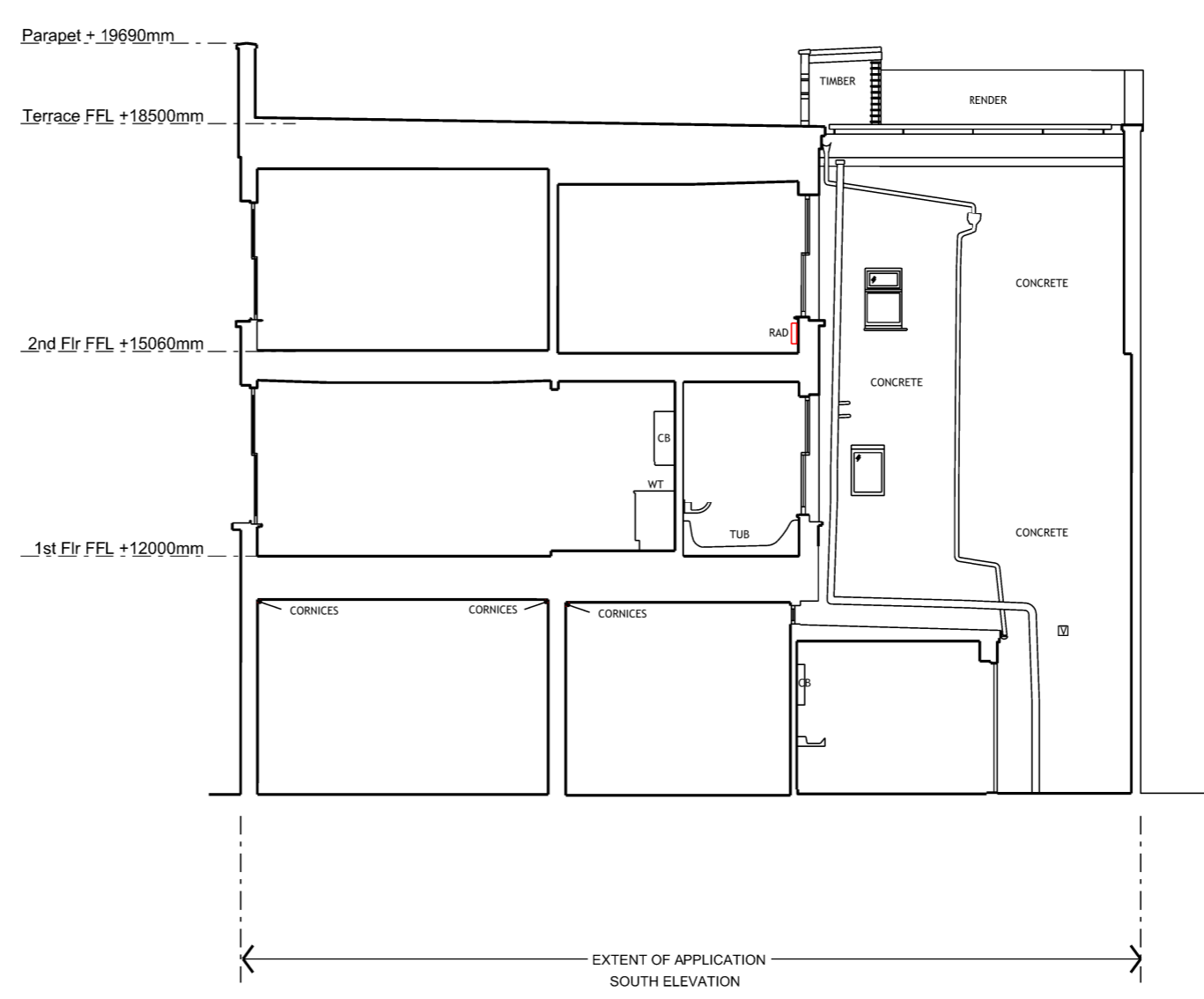
02 SOUTH ELEVATION
